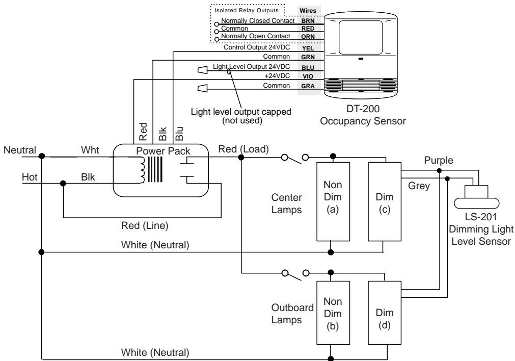
DT-200, LS-201 Wiring Diagram
